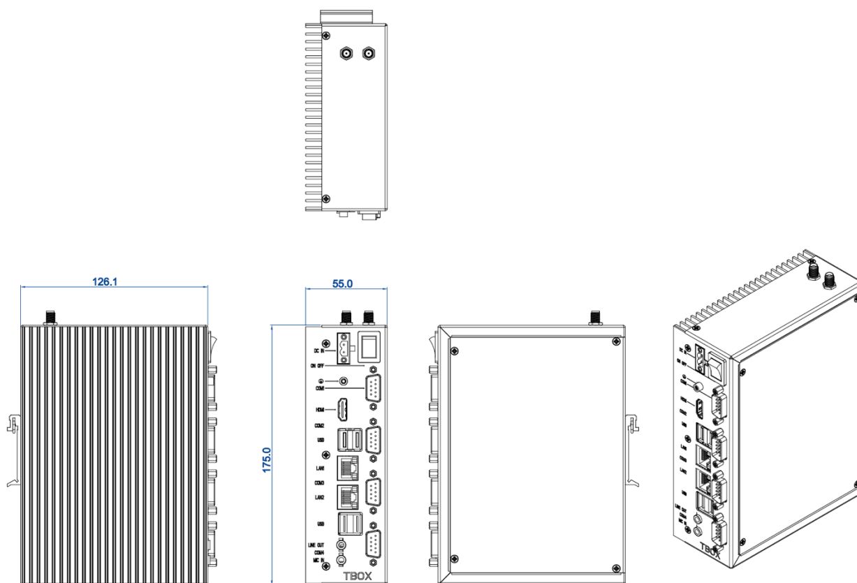
DIMENSIONAL DRAWING:TBOX-1310
